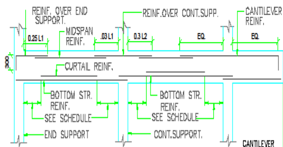
TYPICAL DETAIL OF BEAM REINFORCEMENT.
